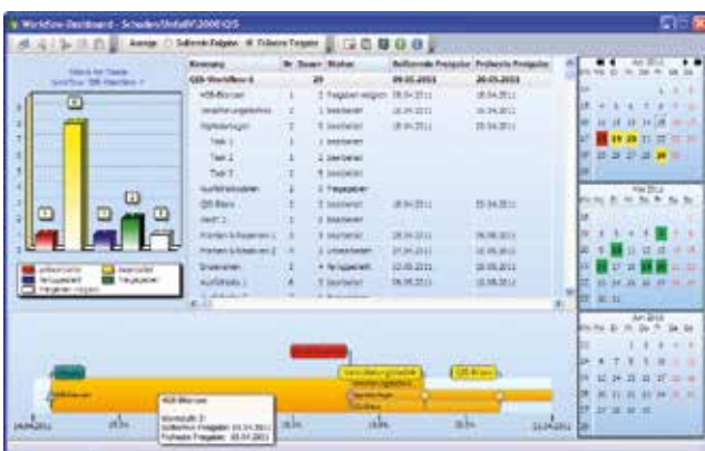
Abb. 4: Workflow-Dashboard
